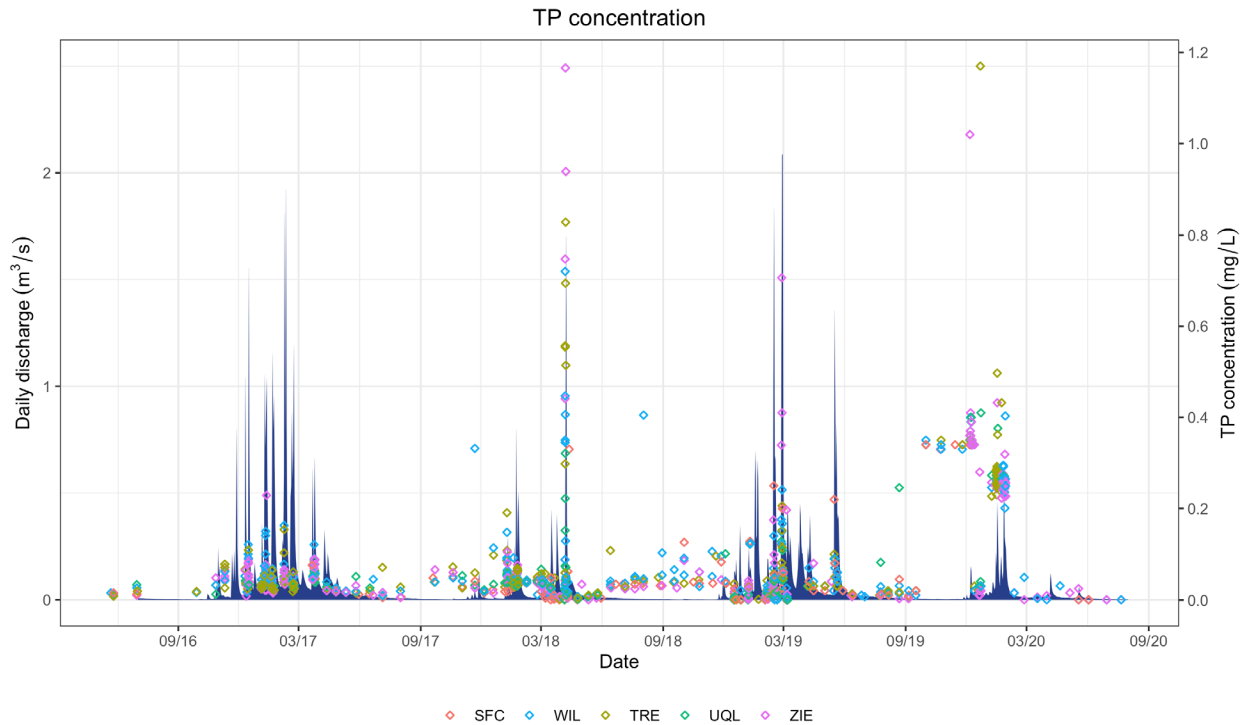
Figure 19: Concentrations of total phosphorus (TP) in stream water in each sub-watershed and South Fork Caspar Creek.
