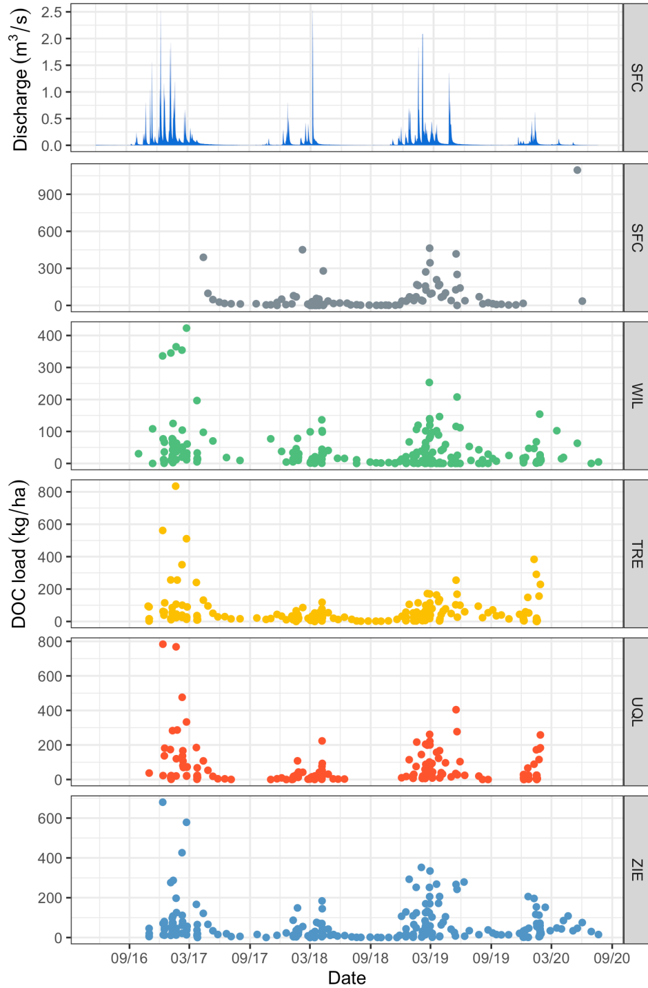
Figure 27: Dissolved Organic Carbon flux in stream water from the treatment sub-watersheds (WIL, TRE, UQL and ZIE) and South Fork Caspar Creek (SFC) for the four year study period. Please note that y-axes differ in range.
