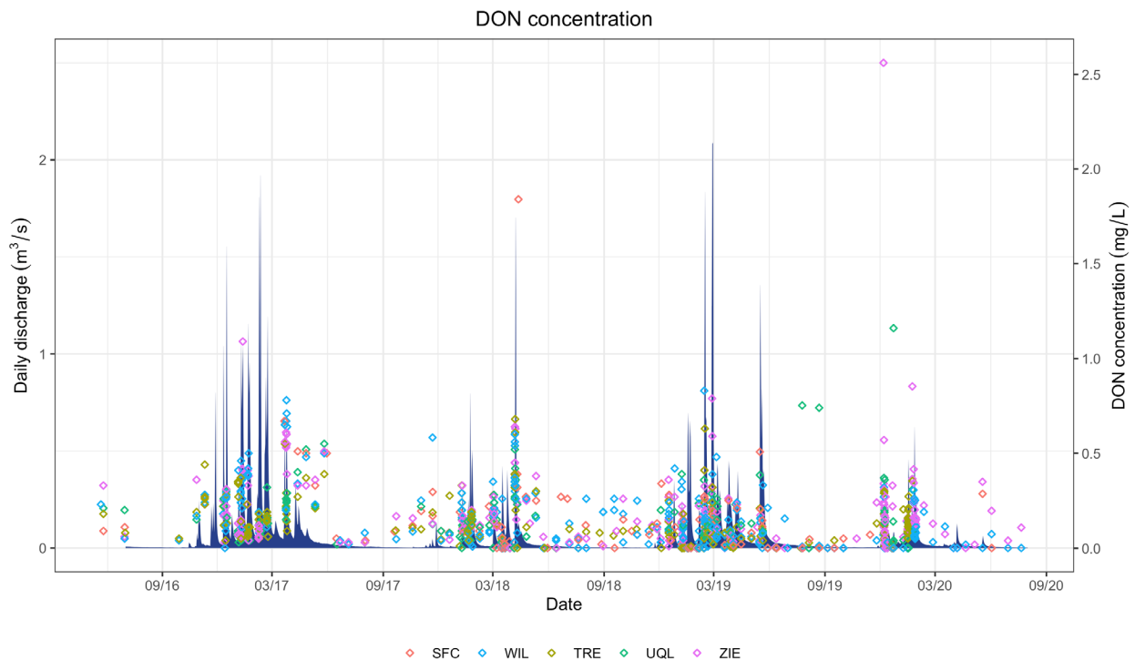
Figure 18: Concentrations of dissolved organic nitrogen (DON) in stream water in each sub-watershed and South Fork Caspar Creek.
