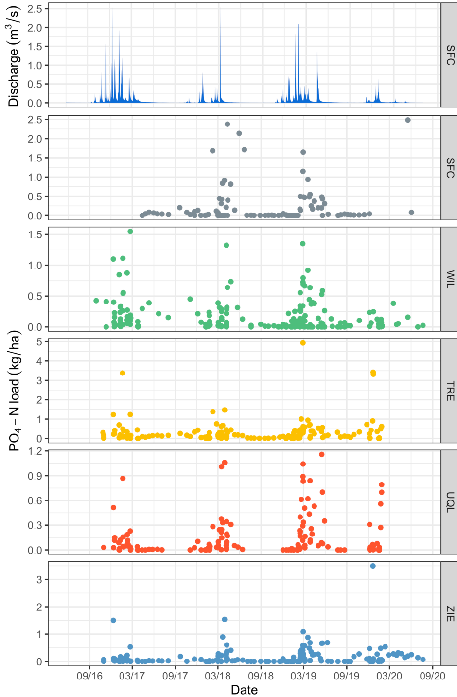
Figure 33: Phosphate flux in stream water from the treatment sub-watersheds (WIL, TRE, UQL and ZIE) and South Fork Caspar Creek (SFC) for the four year study period. Please note that y-axes differ in range.
