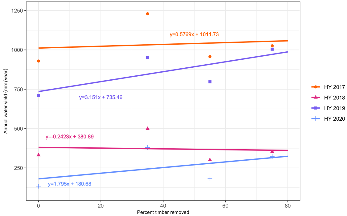
Figure 10: Annual water yield vs. percent timber removed in each watershed comparing hydrological years 2017 – 2020. Hydrologic years 2019 and 2020 are the post-harvest years, while HY 2017 was the wettest year within the 4-year study period.
