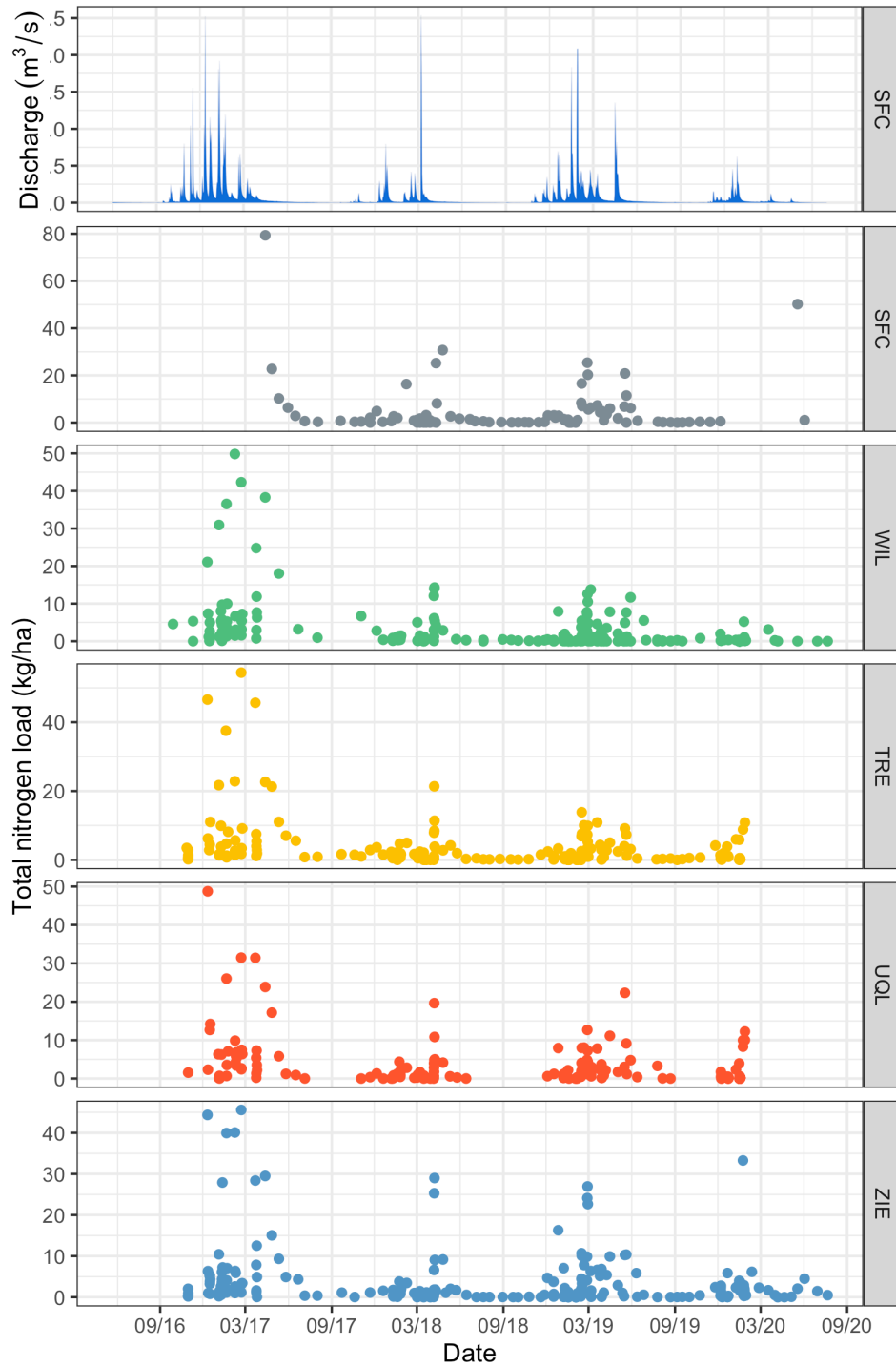
Figure 28: Total nitrogen flux in stream water from the treatment sub-watersheds (WIL, TRE, UQL and ZIE) and South Fork Caspar Creek (SFC) for the four year study period. Please note that y-axes differ in range.
