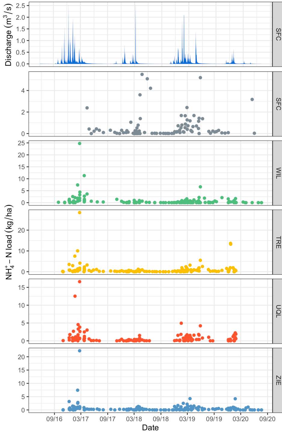
Figure 30: NH 4 + flux in stream water from the treatment sub-watersheds (WIL, TRE, UQL and ZIE) and South Fork Caspar Creek (SFC) for the four year study period. Please note that y-axes differ in range.
