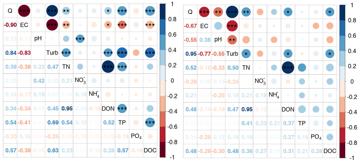
Figure 25: Correlation plot of flow and major water chemistry parameters at ZIE for the pre-tying (left) and post-tying (right) periods. Three, two and one star indicate significant Pearson correlation coefficient at the 0.001, 0.01, and 0.05 significance level, respectively.
