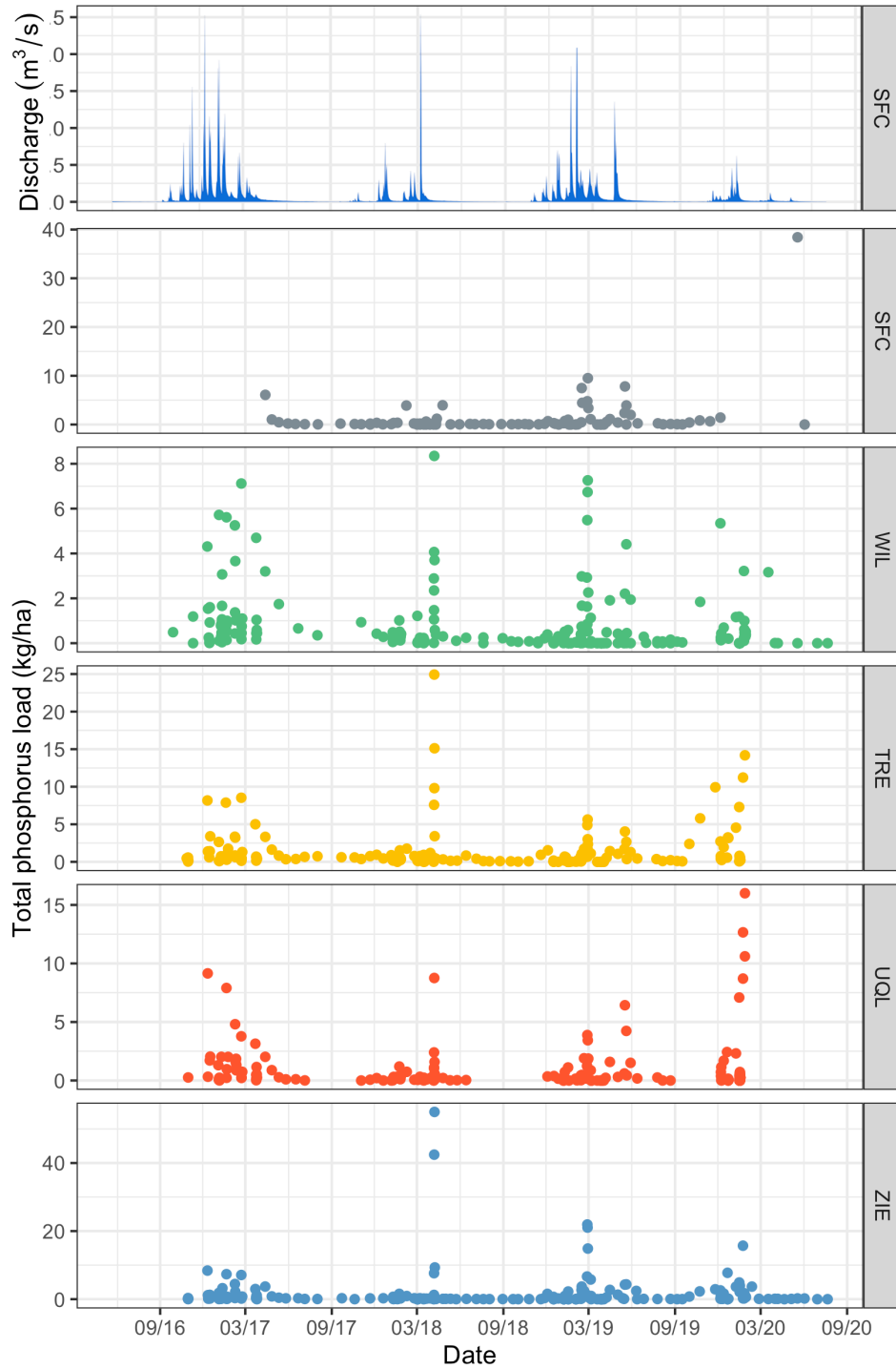
Figure 32: Total phosphorus flux in stream water from the treatment sub-watersheds (WIL, TRE, UQL and ZIE) and South Fork Caspar Creek (SFC) for the four year study period. Please note that y-axes differ in range.
