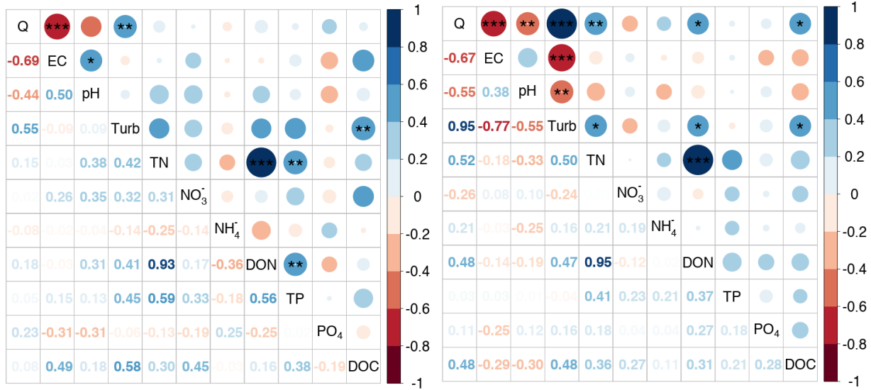
Figure 21: Correlation plot of flow and major water chemistry parameters at SFC for the pre-yrading (left) and post-yrading (right) periods. Three, two and one star indicate significant Pearson correlation coefficient at the 0.001, 0.01, and 0.05 significance level, respectively.
