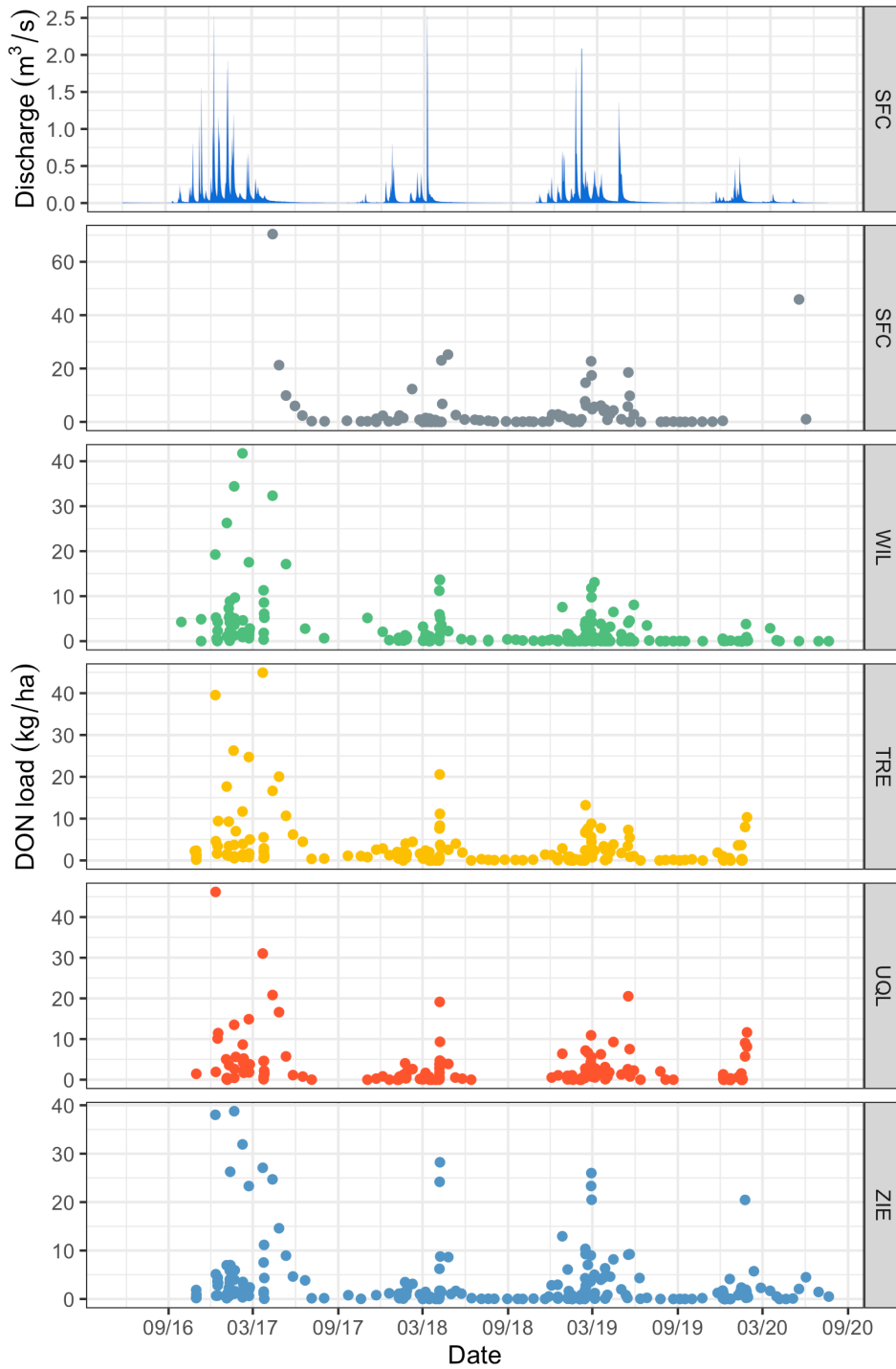
Figure 31: Dissolved Organic nitrogen flux in stream water from the treatment sub-watersheds (WIL, TRE, UQL and ZIE) and South Fork Caspar Creek (SFC) for the four year study period. Please note that y-axes differ in range.
