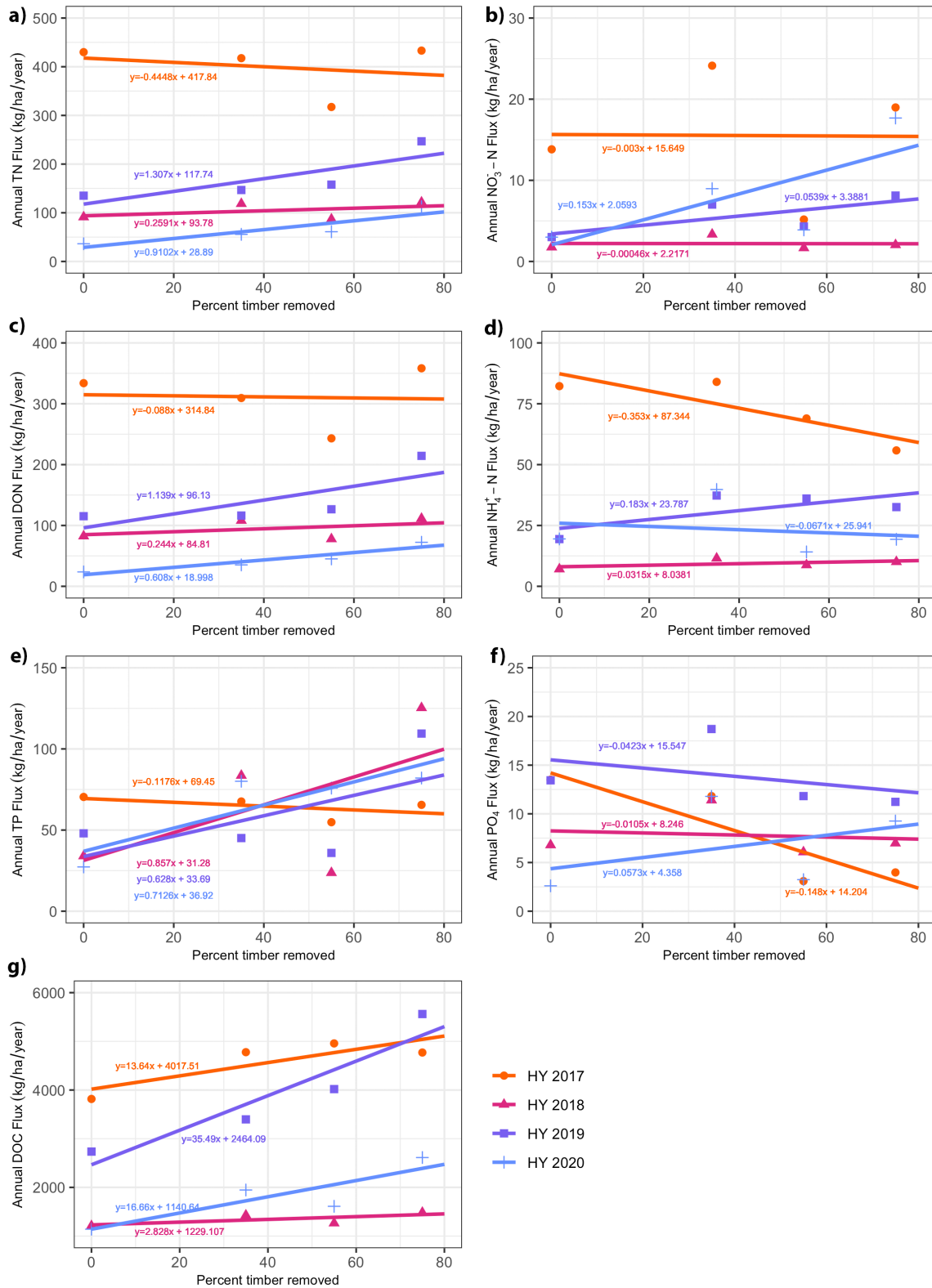
Figure 26: Annual elemental nutrient fluxes (kg/ha/yr) vs. percent timber removed in each sub-watershed for each hydrological year in the 4-year study period. Plots show TN (a), \text{NO}_3^- -N (b), DON (c), \text{NH}_4^+ -N (d), TP (e), \text{PO}_4 -P (f), and DOC (g).
