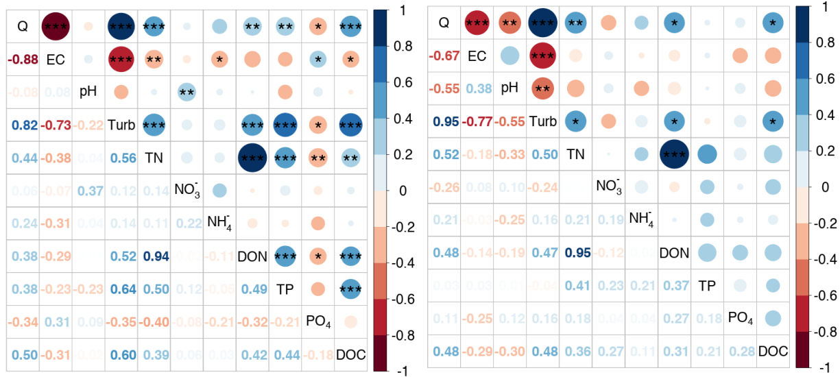
Figure 23: Correlation plot of flow and major water chemistry parameters at TRE for the pre-warding (left) and post-warding (right) periods. Three, two and one star indicate significant Pearson correlation coefficient at the 0.001, 0.01, and 0.05 significance level, respectively.
