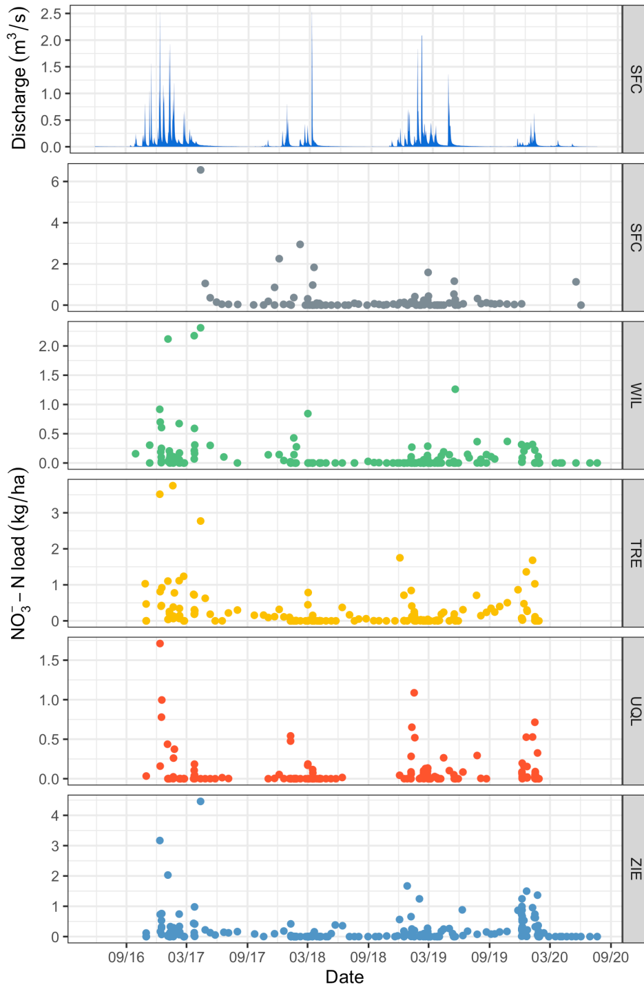
Figure 29: NO 3 - flux in stream water from the treatment sub-watersheds (WIL, TRE, UQL and ZIE) and South Fork Caspar Creek (SFC) for the four year study period. Please note that y-axes differ in range.
