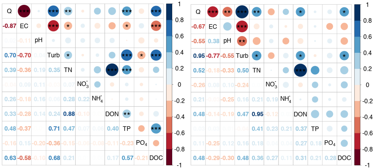
Figure 24: Correlation plot of flow and major water chemistry parameters at UQL for the pre-warding (left) and post-warding (right) periods. Three, two and one star indicate significant Pearson correlation coefficient at the 0.001, 0.01, and 0.05 significance level, respectively.
