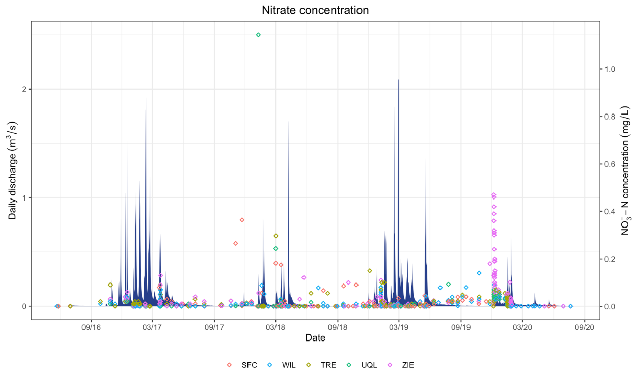
Figure 16: Concentrations of nitrate-nitrogen ( \text{NO}_3^- -N) in stream water in each sub-watershed and South Fork Caspar Creek.
