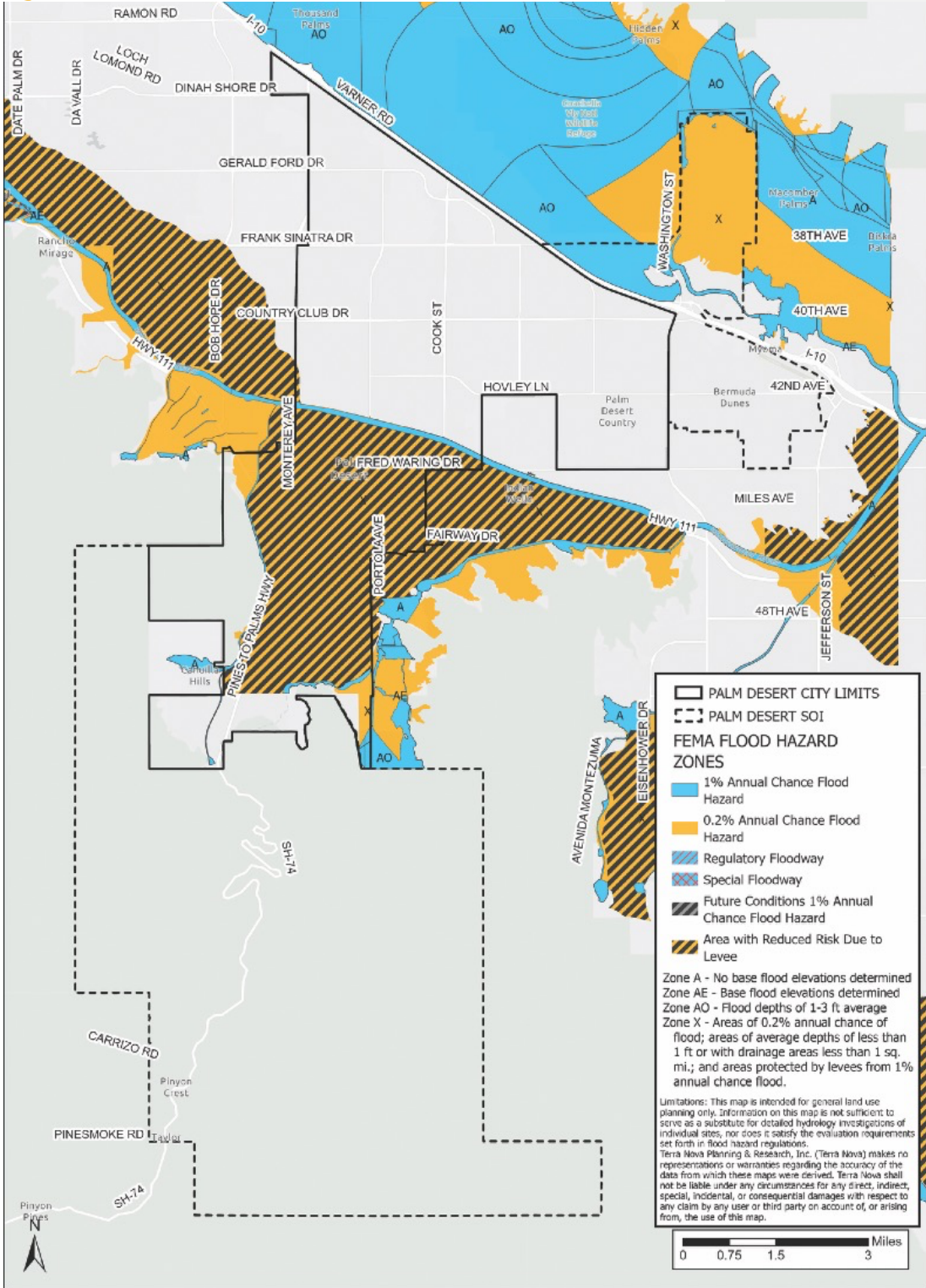
Figure 8.4 FEMA Flood Zones
