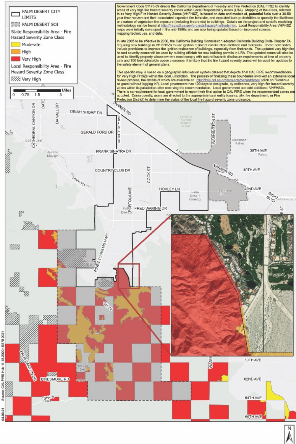
Figure 8.5 Fire Hazard Severity Zones
