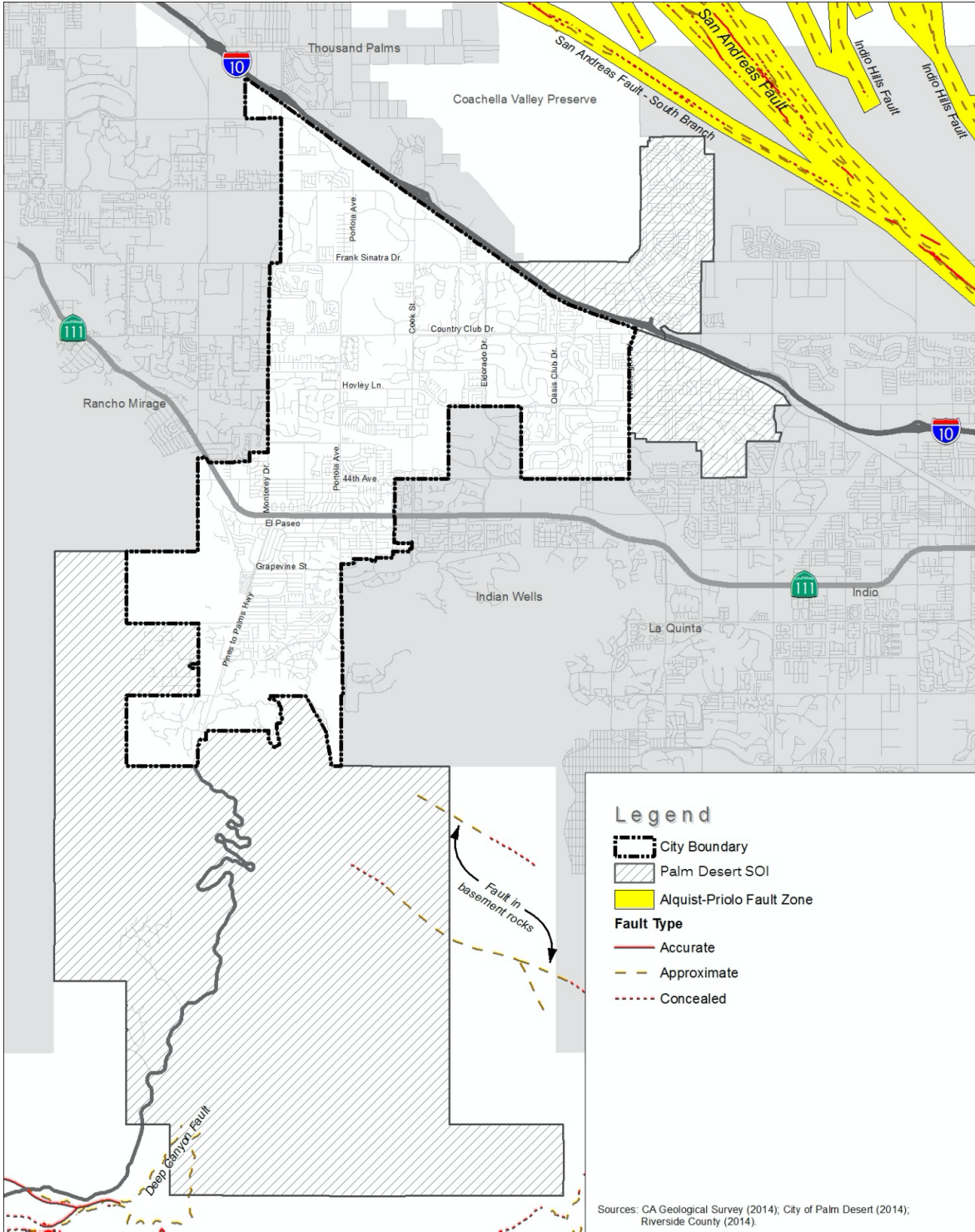
Figure 8.1 Faults and Fault Zones in Palm Desert
