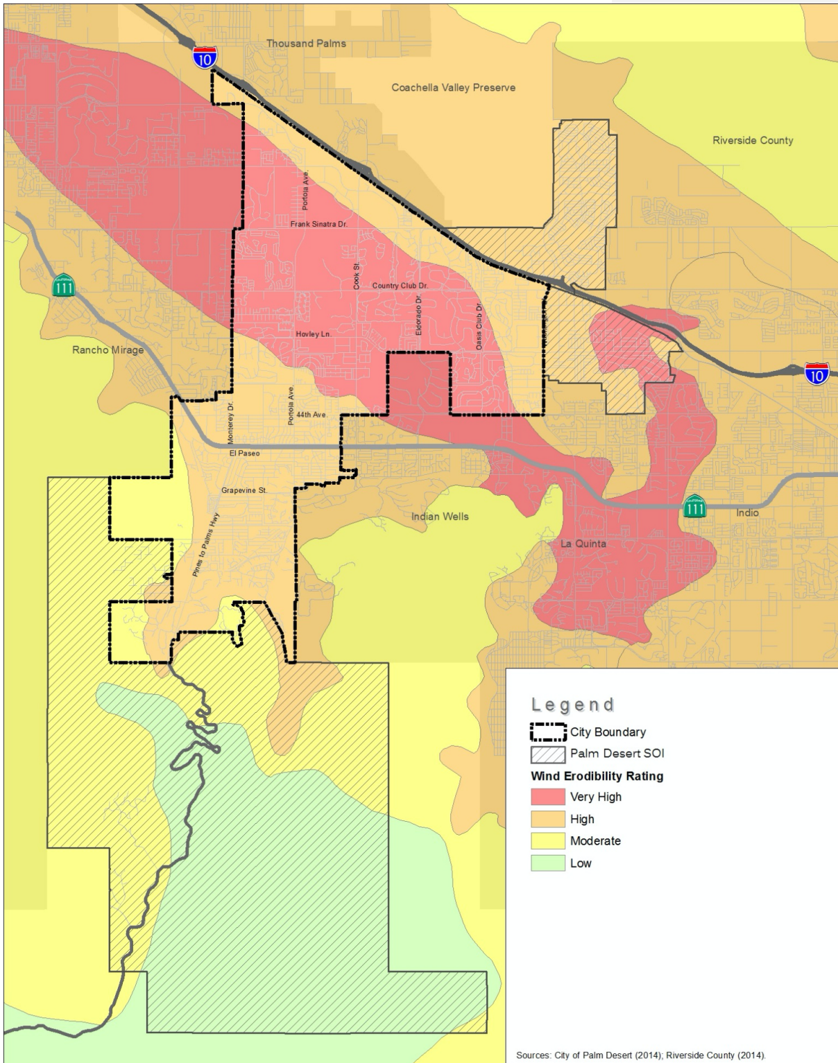
Figure 8.3 Wind Erosion Hazard
