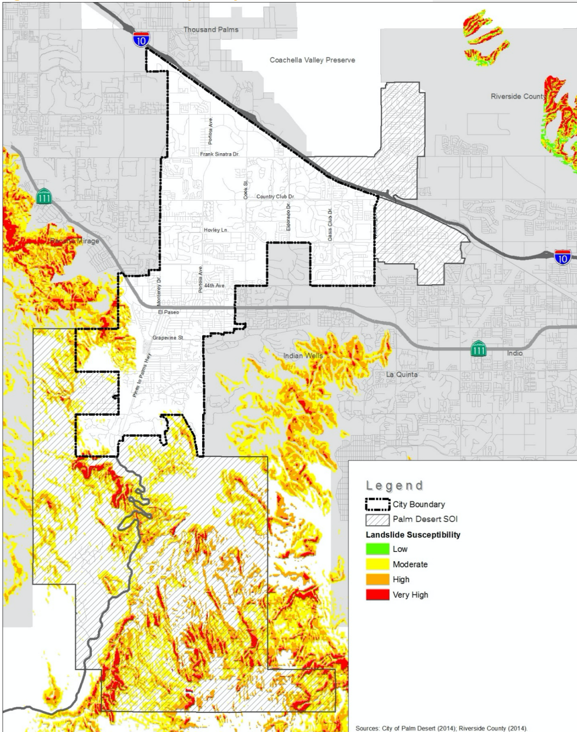
Figure 8.2 Landslide Susceptibility
