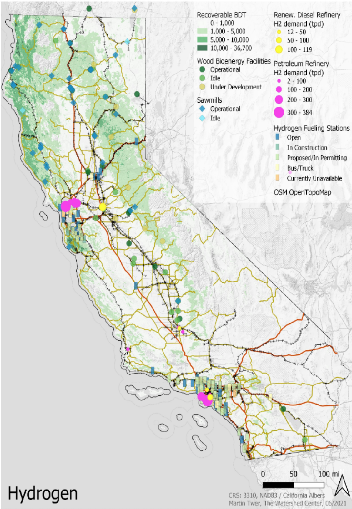
Figure 2: The potential supply chain for hydrogen in California (Credit: Martin Twer, the Watershed Center, 06/2021)
