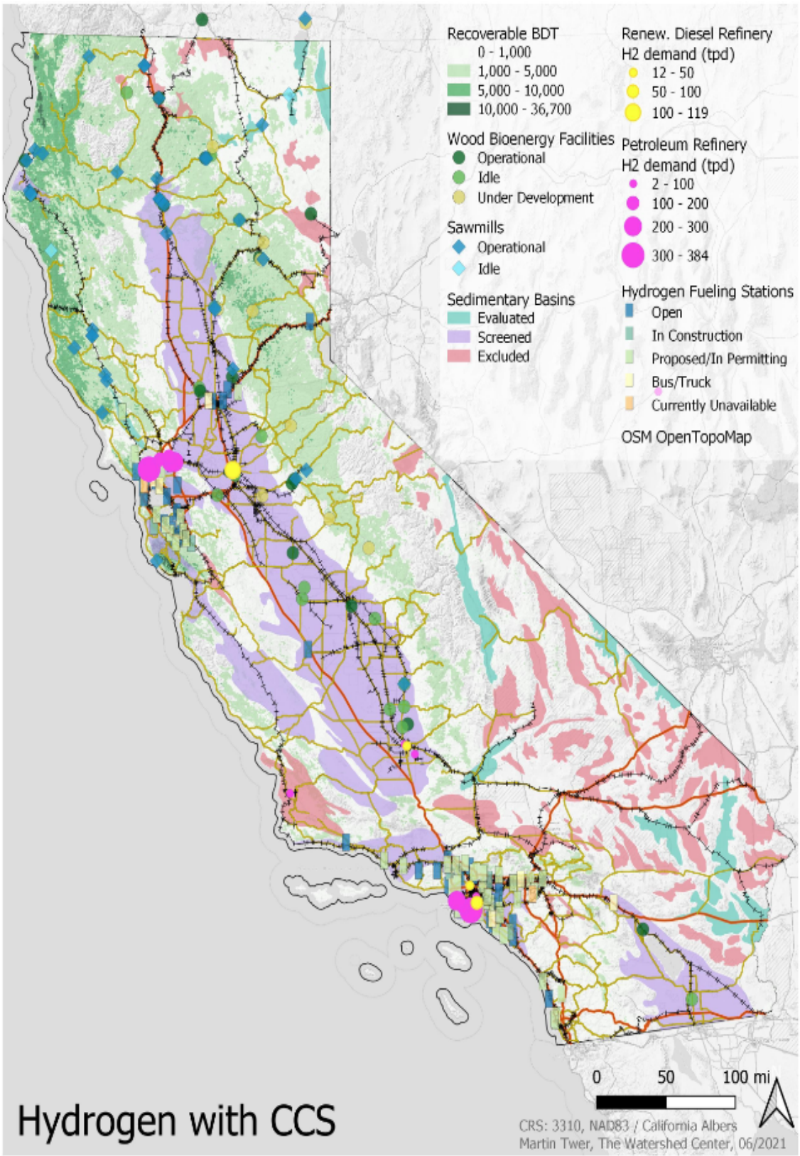
Figure 3: The potential supply chain for hydrogen with CCS in California
