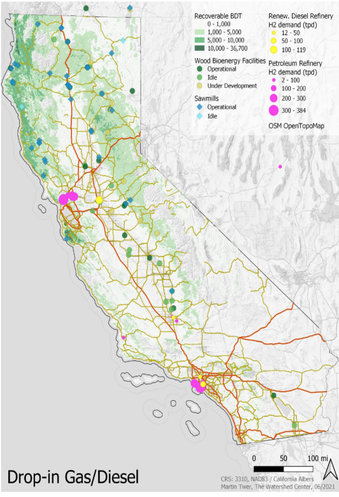
Figure 6: The potential supply chain for drop-in gas/diesel in California
