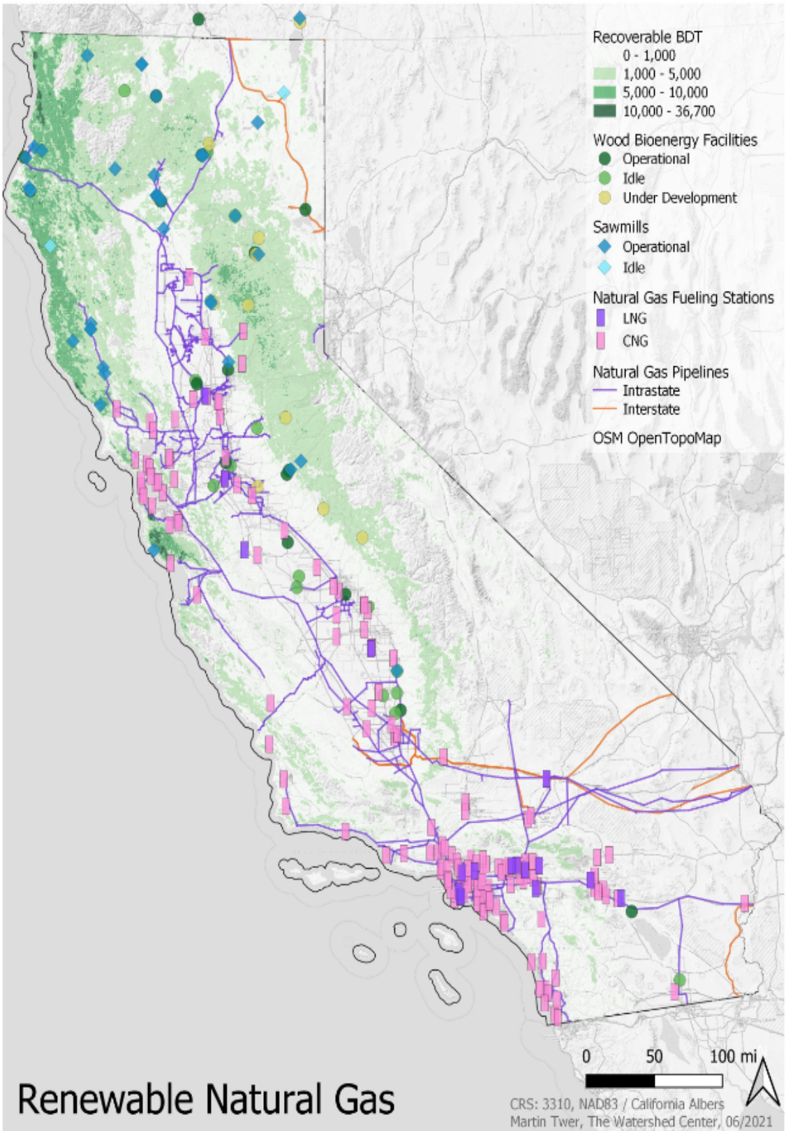
Figure 7: The potential supply chain for RNG in California
